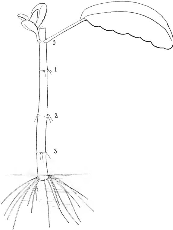
FIG. 91.—Growth of shoot is more rapid in Fig. 91 than in Fig. 92, p. 117.
